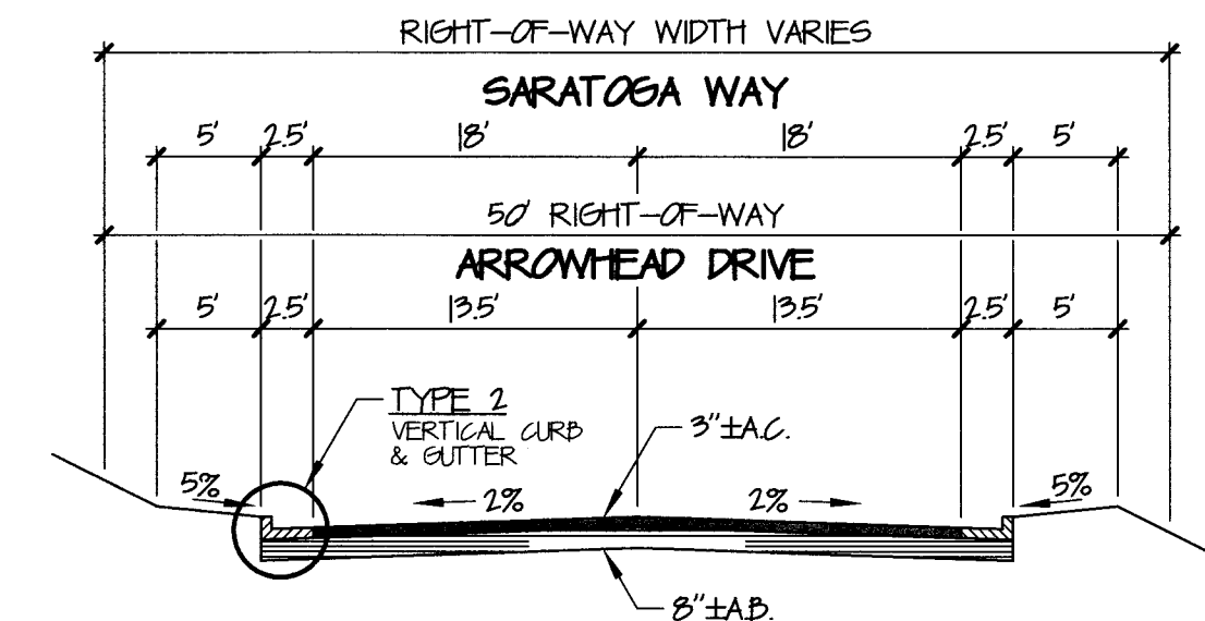
TYPICAL STREET SECTION EXISTING COUNTY ROADS NOT TO SCALE
